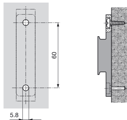
Fig. 4. Drilling pattern.
