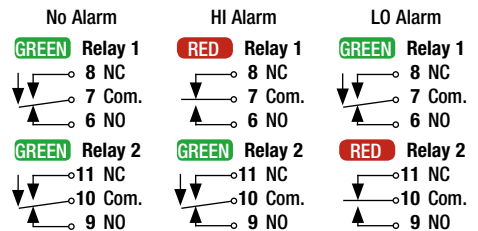
API 1025 G Alarm States with Normal Action HI/LO Alarms
