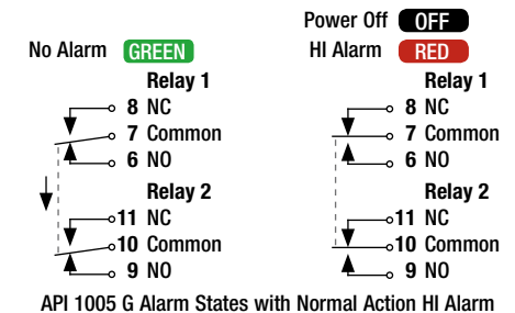
API 1005 G Alarm States with Normal Action HI Alarm
