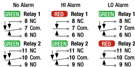
API 1020 G Alarm States with Normal Action HI/LO Alarms
