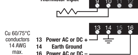
Thermistor Input
