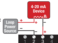
Current Sinking Output switch E set to "I" External loop supply
