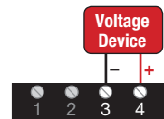
Voltage Output Switch E set to "V"
