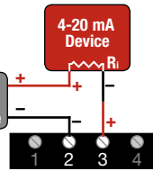
Current Sinking Output switch E set to "I" External loop supply Module mA output is unpowered
