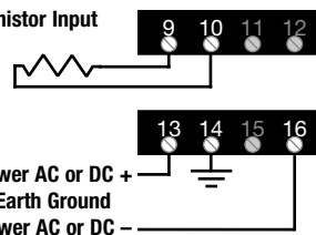
Thermistor Input
