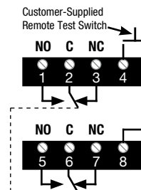
Relay Wiring APD 1600
