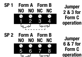
Relay Wiring APD 1421, 1431
