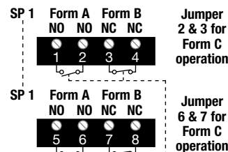
Relay Wiring APD 1401
