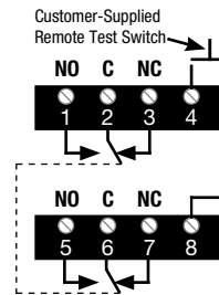
Relay Wiring APD 1400
